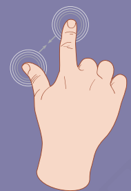
Zooming
