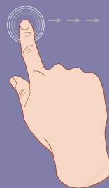
Dragging
