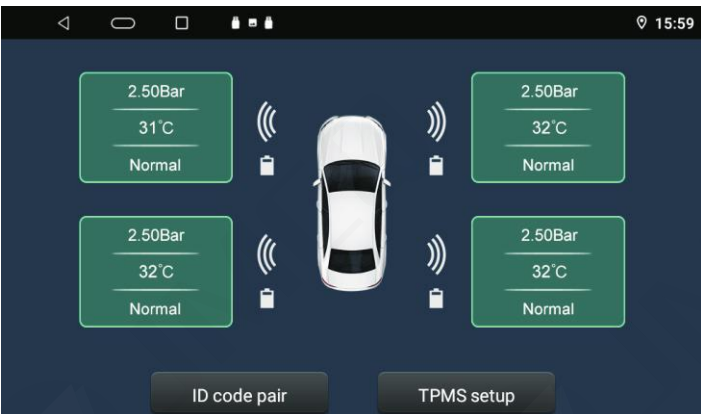
7. Use interface.
